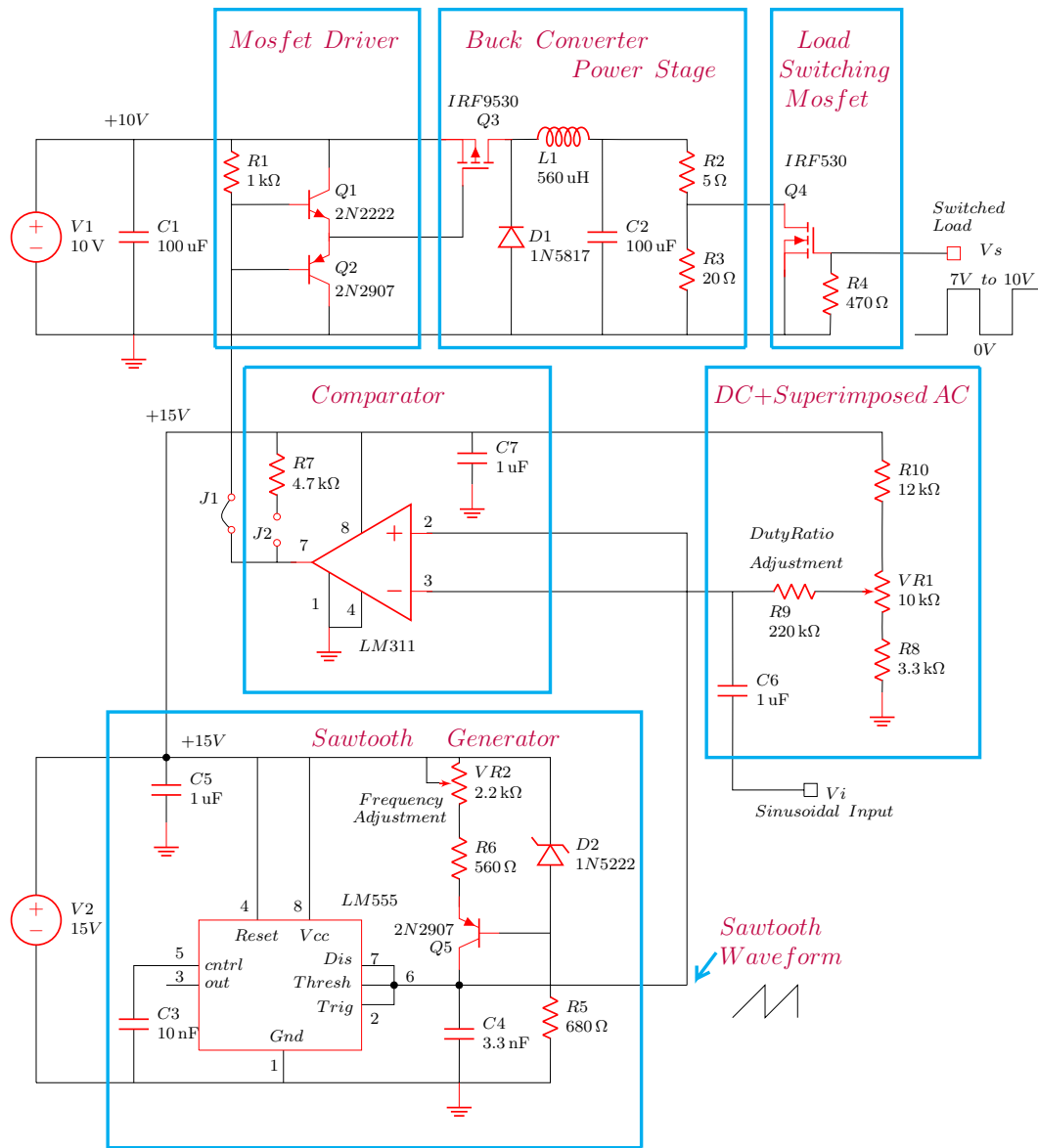
Figure 14.2: Schematic of the open-loop dc-to-dc buck converter.
