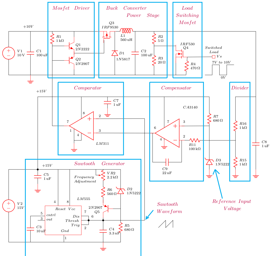
Figure 15.8: Schematic of the closed-loop voltage regulator system.
